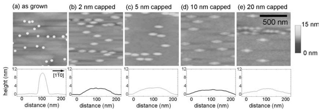
Figure 4.7 1 \times 1 \mu\text{m}^2 AFM images of the 1.8 ML InAs QDs with thin GaAs capping layer thicknesses: (a) as grown, (b) 2-nm capped, (c) 5-nm capped, (d) 10-nm capped, (e) 20-nm capped. The bottom row shows the cross-sectional view of a nanostructure. The shape of the QDs drastically changes during the capping process.
