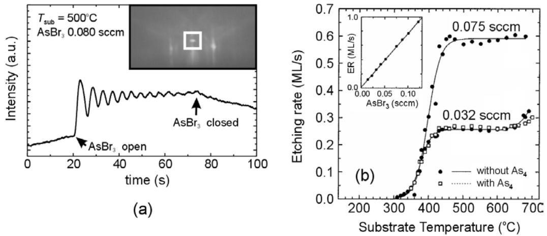
Figure 3.7 (a) RHEED oscillation result obtained during the etching of GaAs by AsBr 3 at 500°C. The intensity signal is obtained from the white box shown in the inset. (b) The etching rate obtained from RHEED intensity oscillation versus substrate temperature for two different AsBr 3 flow rates. For 0.032 sccm AsBr 3 flow rate, the etching rates with and without a concomitant As flux are shown. In the lower temperature region from 300 to 420°C, the etching is reaction-rate-limited ; in the upper temperature region above 450°C it is supply-rate-limited . The etching rate in the supply-rate-limited regime, as a function of AsBr 3 flow rates, is shown in the inset (Ritz et al., 1997).
